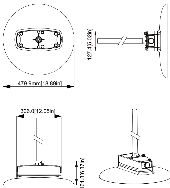
G3/4" NPT Pole Mounting
