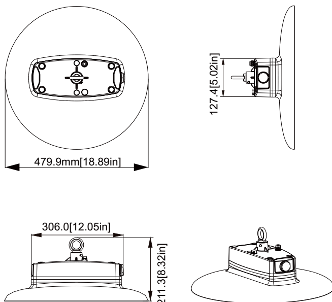
Hanging Rings Mounting
