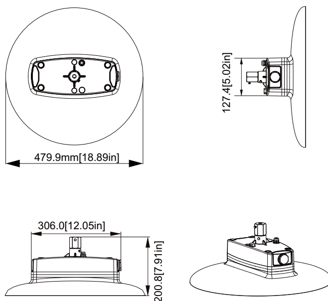
With G3/4" NPT to M12 adapter Mounting
