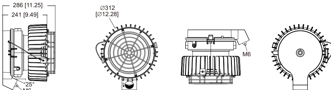
Q2 with driver cover D, wire guard, and flat diffuser
